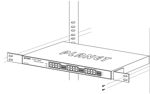
Figure 5: Mounting the Gigabit Ethernet Switch in a Rack
