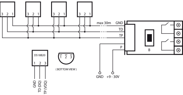
Diagram 4 – Connection to DS18B20 sensors
