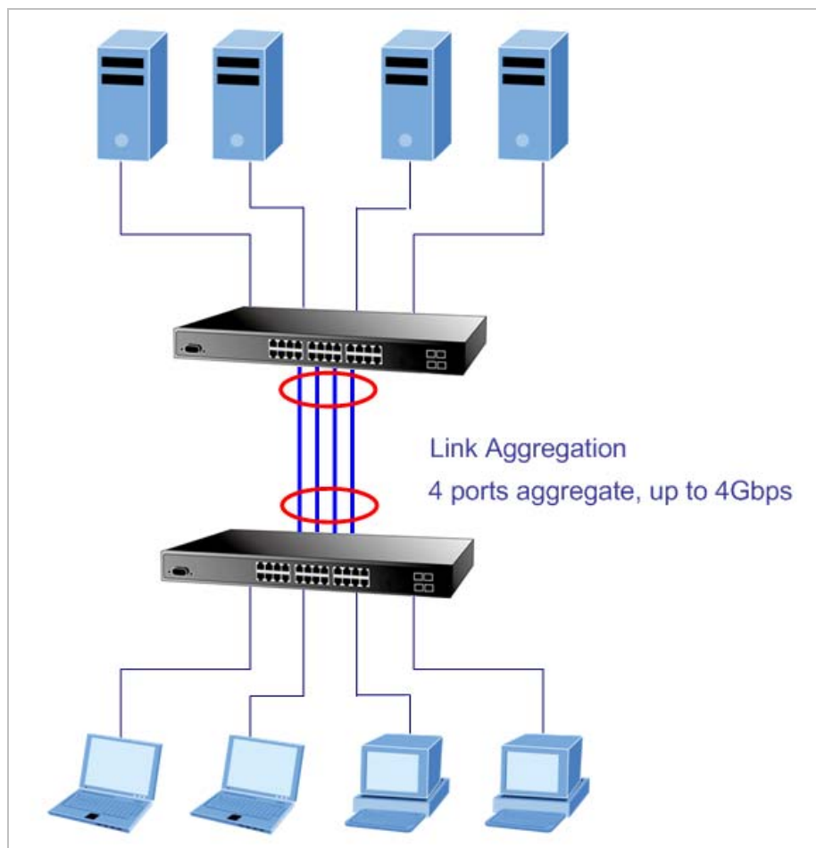
Figure 4-5-1 Link Aggregations
