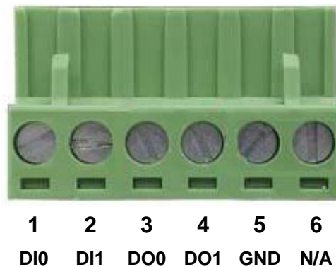
Figure 2-12 6-Pin Terminal Block DI / DO Wiring Input
