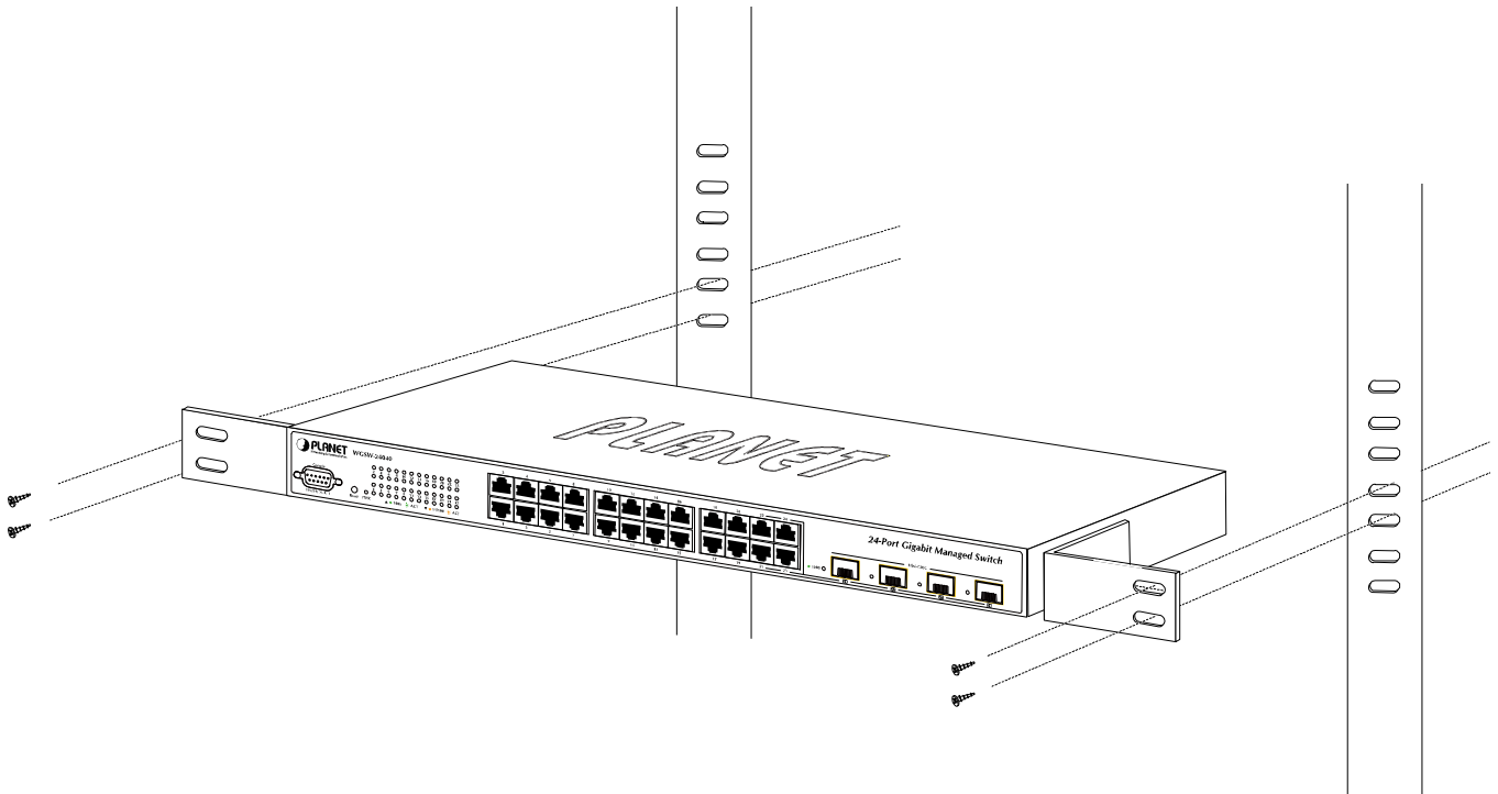
Figure 2-6 Mounting the Managed Switch on a Rack
