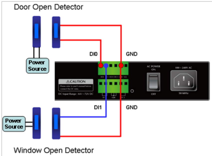
Figure 2-13 Wires DI0 and DI1 to Open Detector
