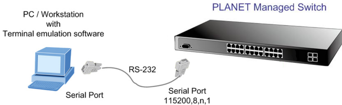
Figure 3-1 Console Management Diagram
