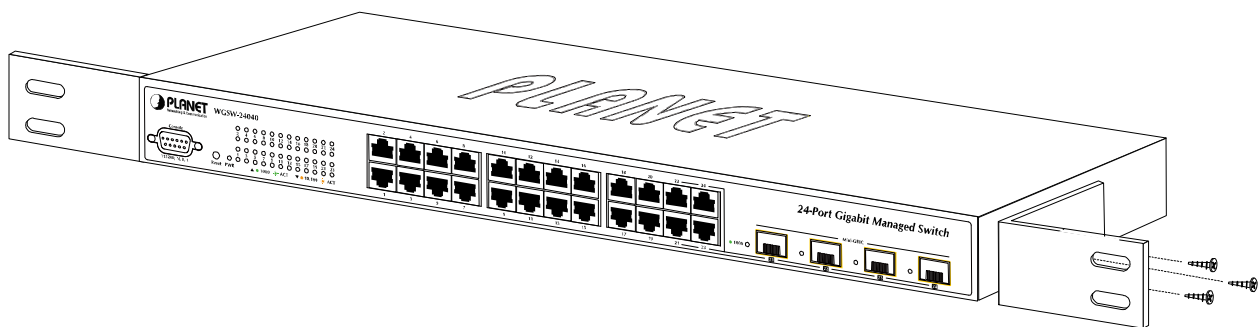
Figure 2-5 Attach Brackets to the Managed Switch.
