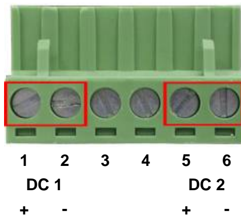
Figure 2-10 6-Pin Terminal Block Power Wiring Input
