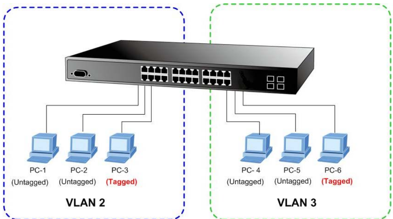
Figure 4-6-8 two separate VLAN Diagram
