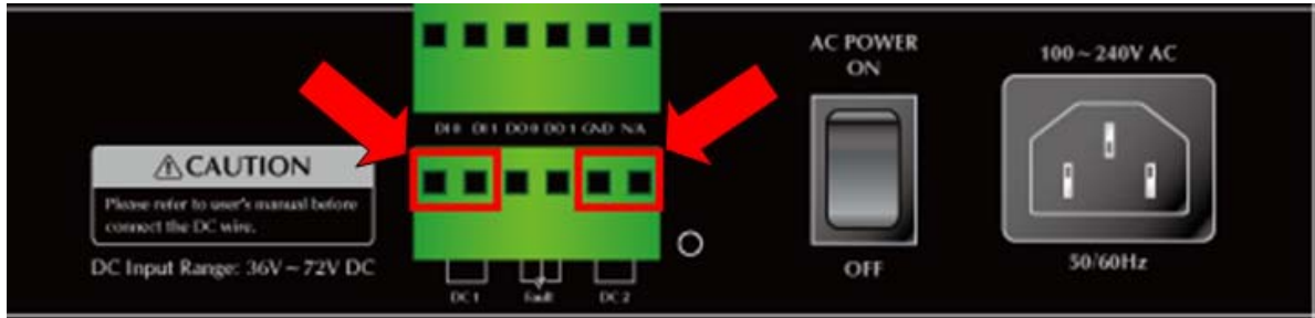
Figure 2-9 Wiring the Redundant Power Inputs
