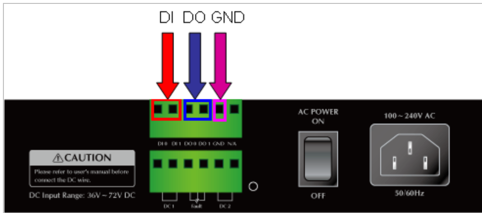
Figure 2-11 Wiring the Redundant Power Inputs
