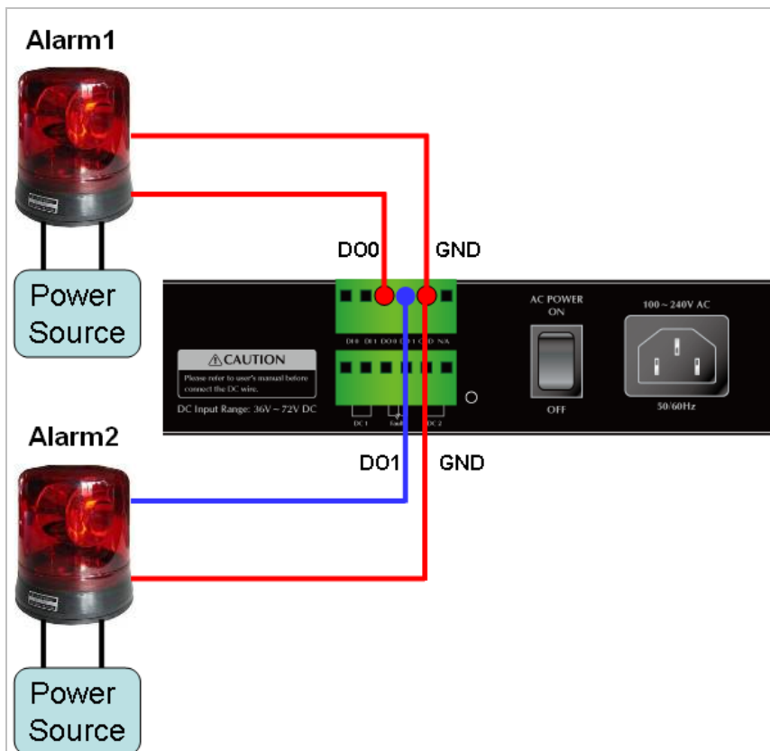
Figure 2-14 Wires DO0 and DO1 to Open Detector
