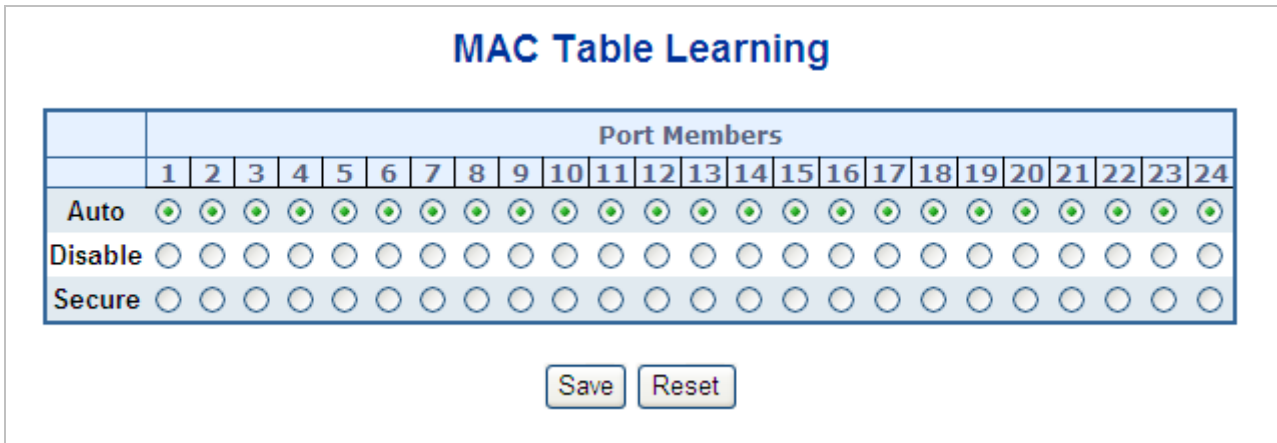
Figure 4-13-4 MAC Table Learning Page Screenshot
