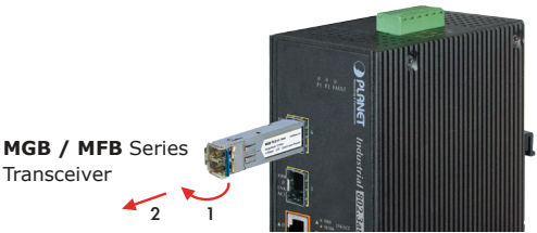
Figure 2-4: Pulling out from the transceiver
