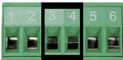
Figure 4: Fault Pin of Terminal Block.
