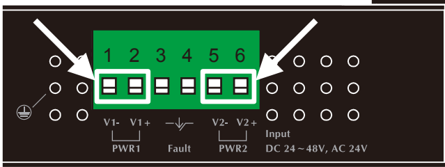
Figure 2: Power input PINs.
