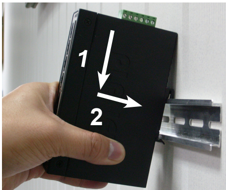
Figure 6: Install Industrial Equipment in DIN-Rail mount.
