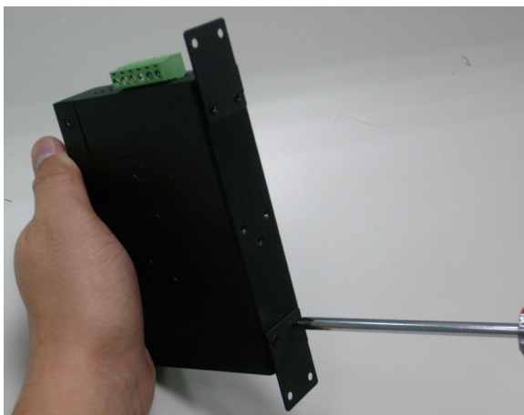
Figure 9: Attach Brackets to the Industrial Equipment.
